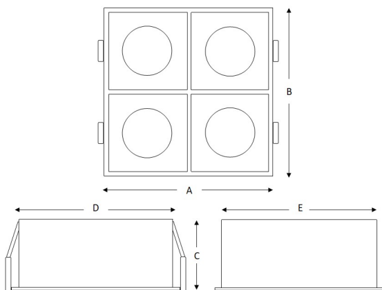
Sizes drawing
