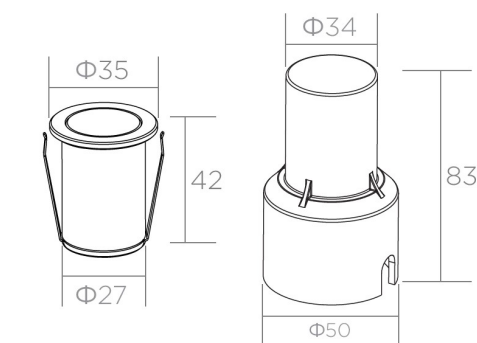
Sizes in mm
