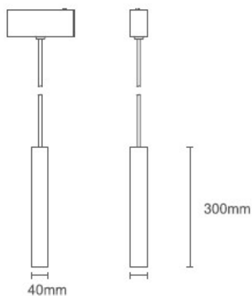
Sizes drawing
