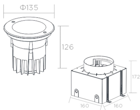
Sizes in mm
